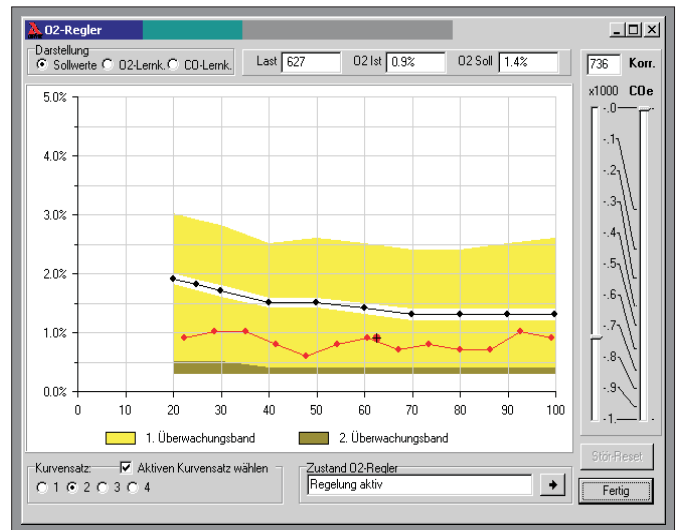
Figure 3: Visualisation of the O 2 /CO setpoint-curve with its monitoring-band-gaps when using the ETAMATIC's OEM integrated O 2 /CO control
