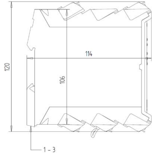
Fig. 1-2 dimensions F130I Housing material: Plastic
