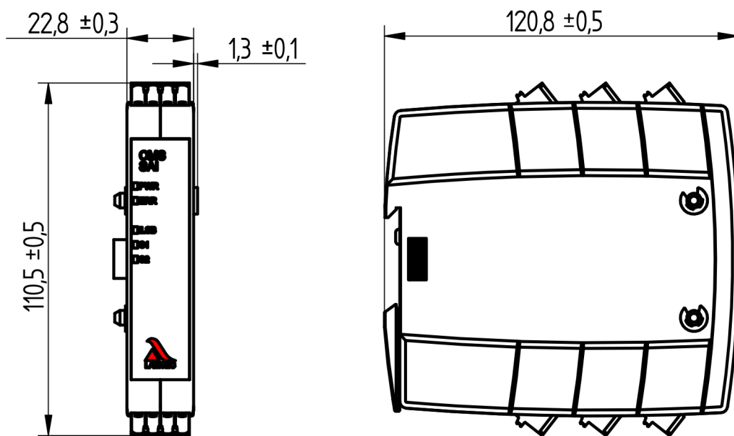
Fig. 2 SAI dimensional drawing
