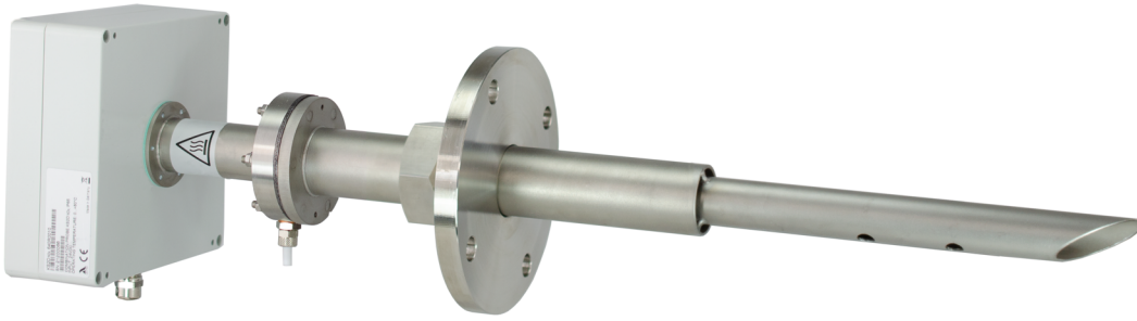
Fig. 3 Combination Probe KS2DNO x with gas extraction device GED FLEX
