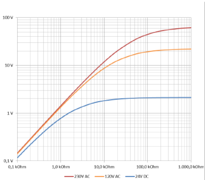
Fig. 6 Residual voltage with output in off-state
