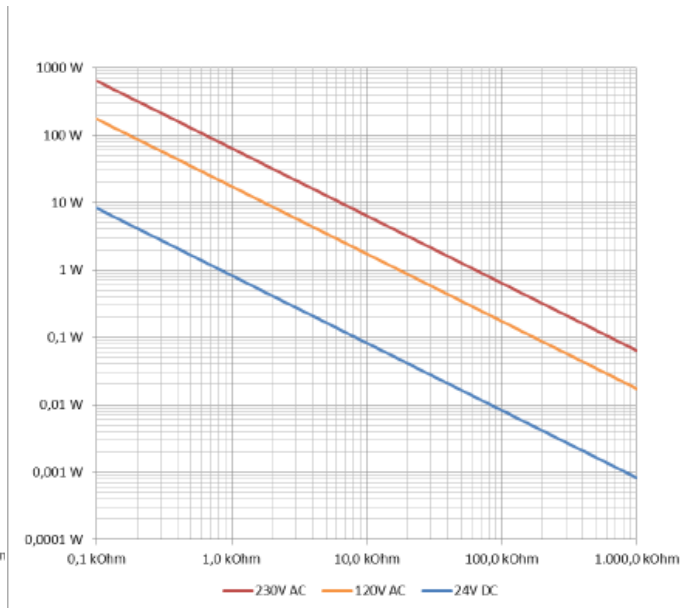
Fig. 7 Power of the additional resistor with output switched on
