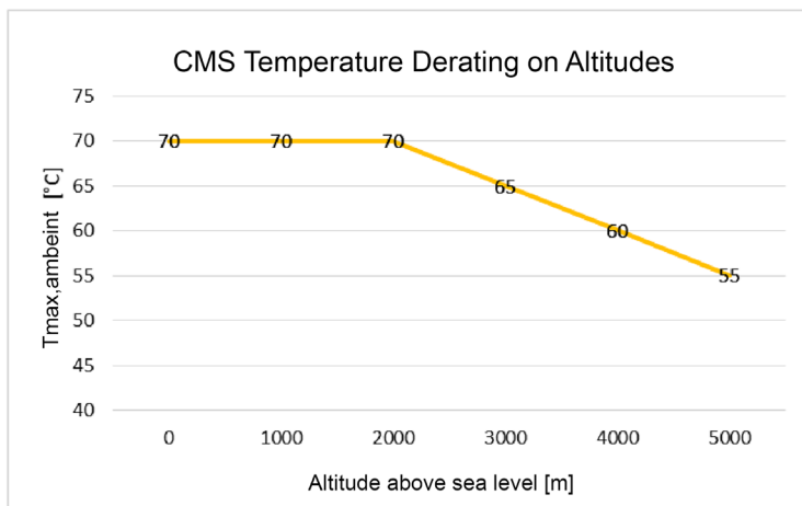
Fig. 5 Temperature underload for use >2000m above sea level
