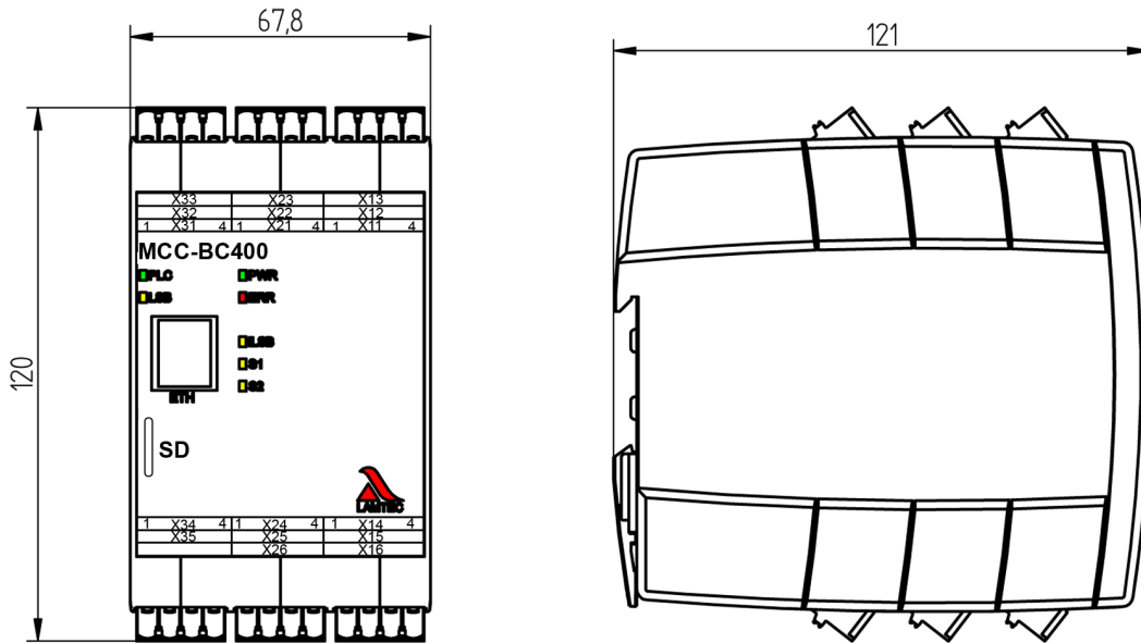
Fig. 4 MCC-BC400 dimensional drawing
