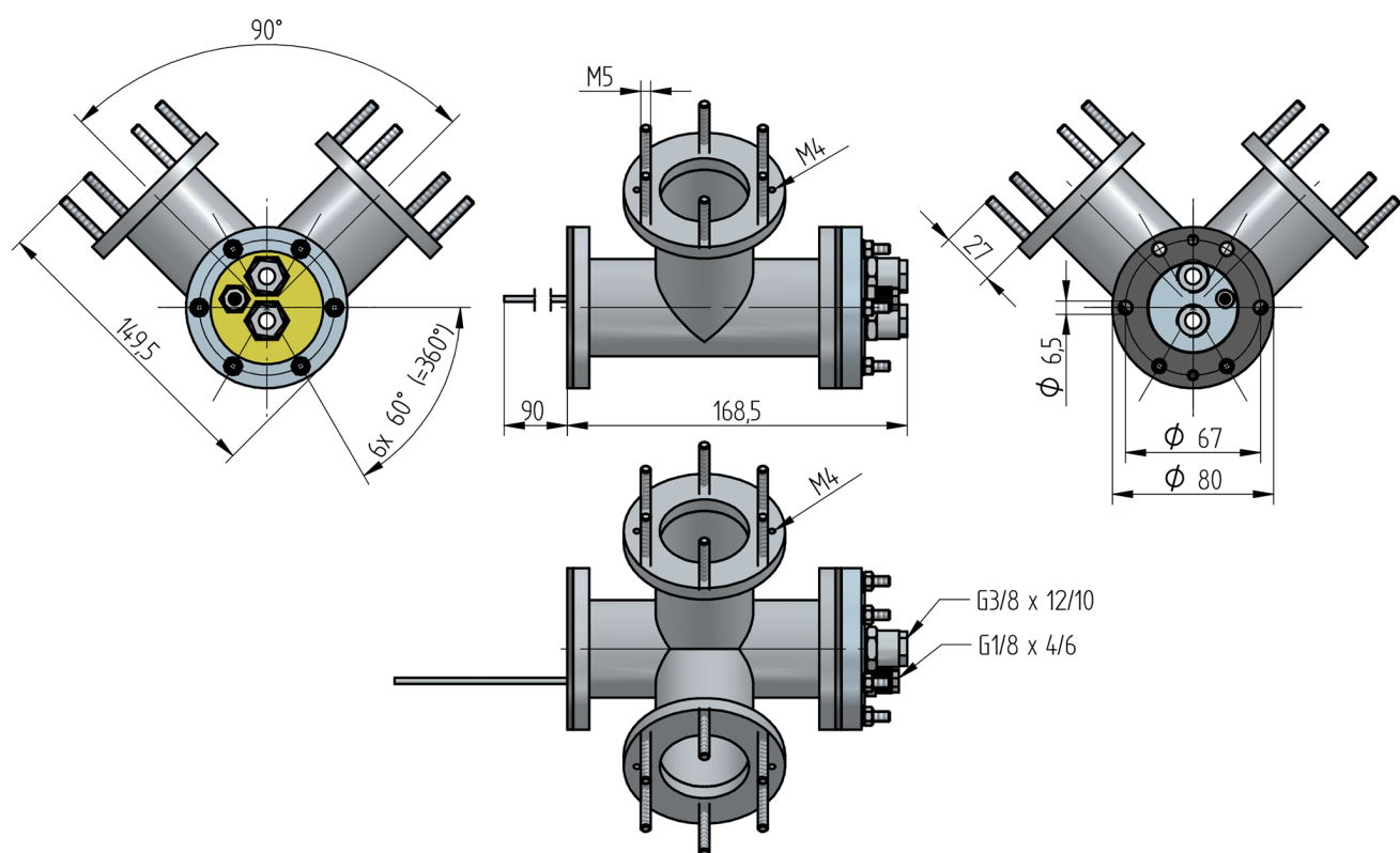
Fig. 1 V-adapter for probe mounting for purge operation and injector acceleration
