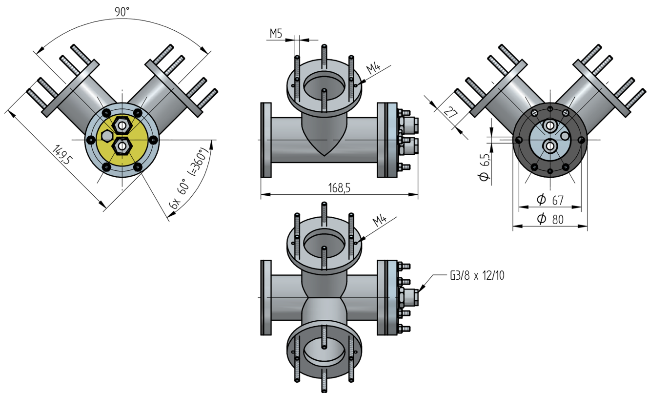
Fig. 1 V-adapter for probe mounting for purge operation inside/outside
