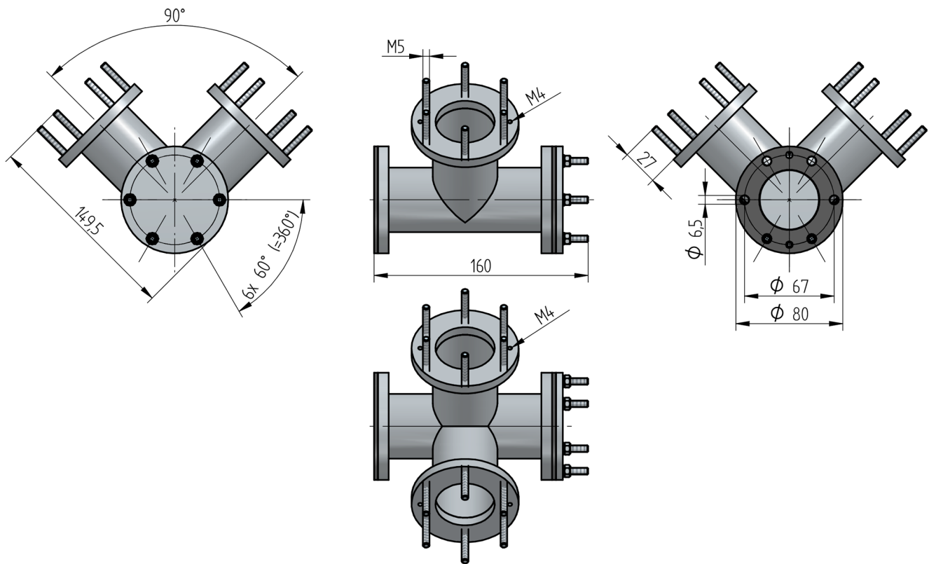
Fig. 1 V-adapter for blind flange
