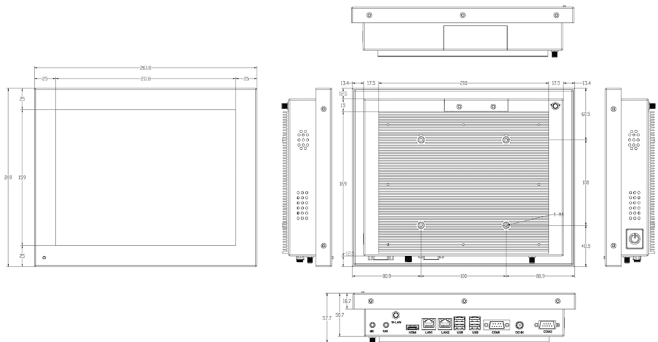
Fig. 2 Dimension GKI300
