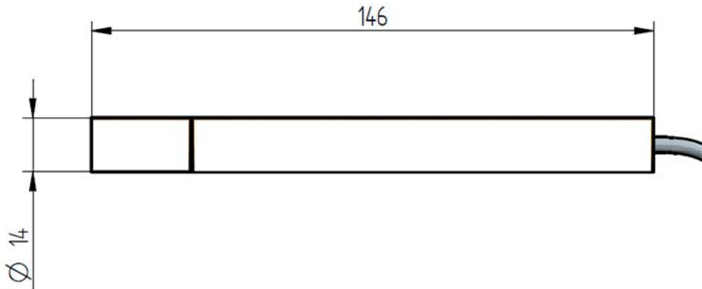
Fig. 1 CarboSen HT
