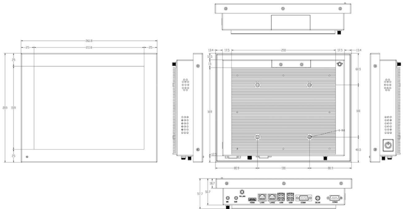
Fig. 2 Dimensions GKI300
