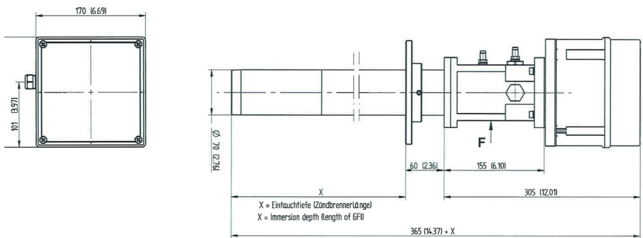
Fig. 4 Dimensions of GFI70 pilot burner Ex-Zone 2
