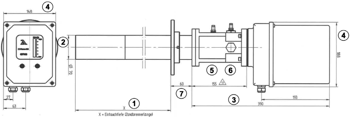
Fig. 2 Dimensions of GFI70 pilot burner design A/B
