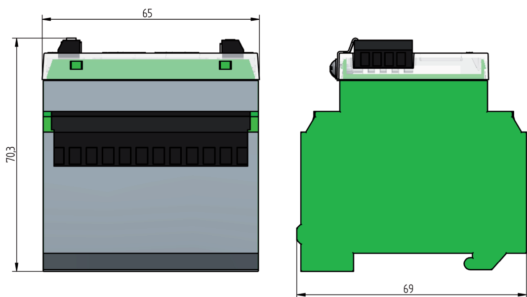
Fig. 1 Dimensions CMS /EBM412
