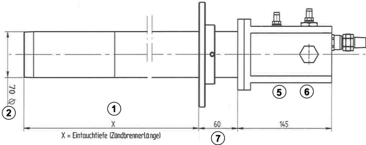
Fig. 6 Dimensions of GF170 pilot burner design C
