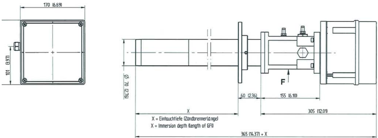
Fig. 4 Dimensions of GF170 pilot burner Ex-Zone II
