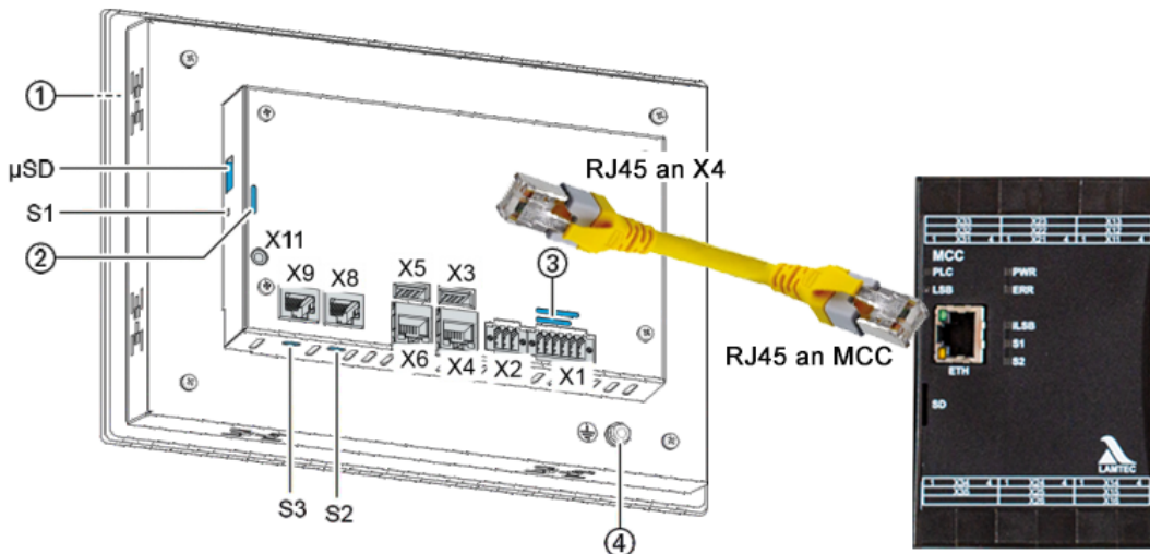
Fig. 5 Anschlüsse GUI615
