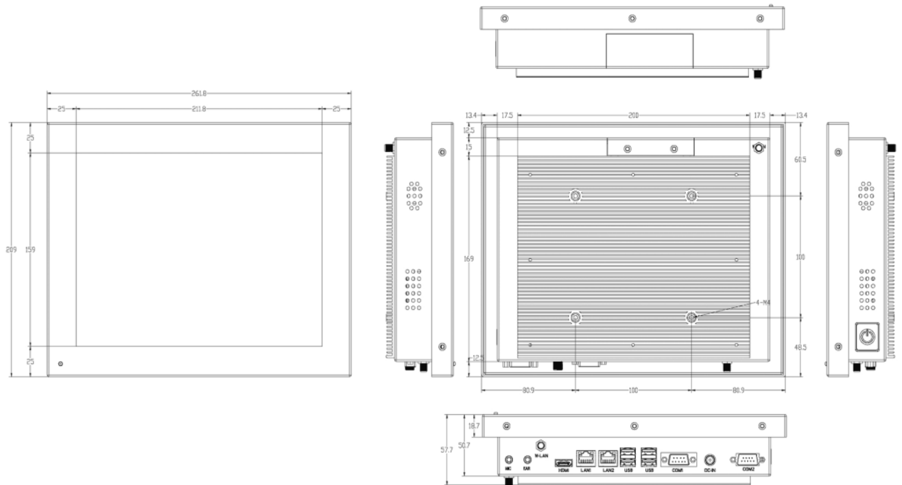
Fig. 1-2 Dimensions GKI300
