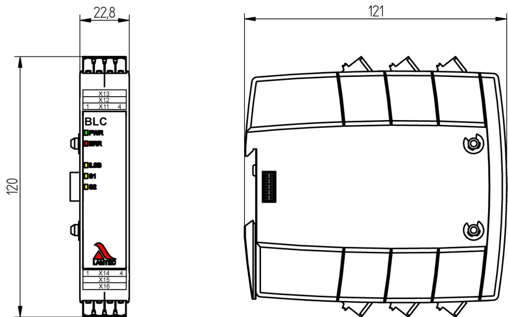
Fig. 2 BLC dimensional drawing
